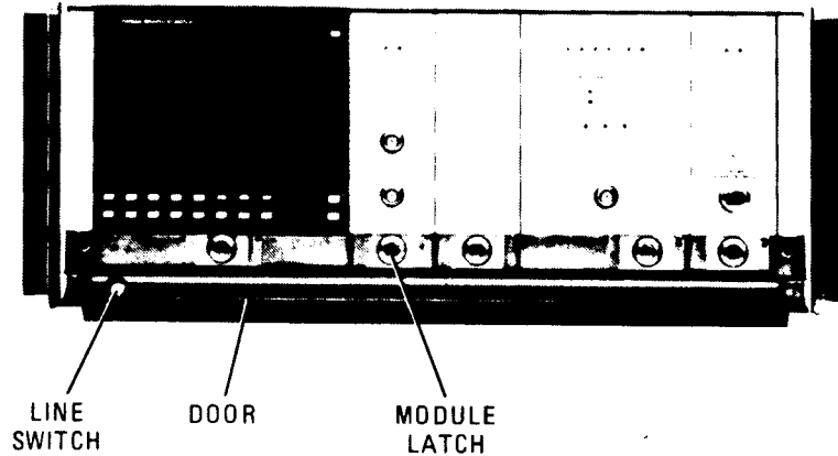
Figure 2-3. Module Installation
